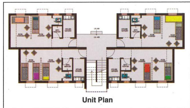
Fig. 15 Typical Plan of A Unit
