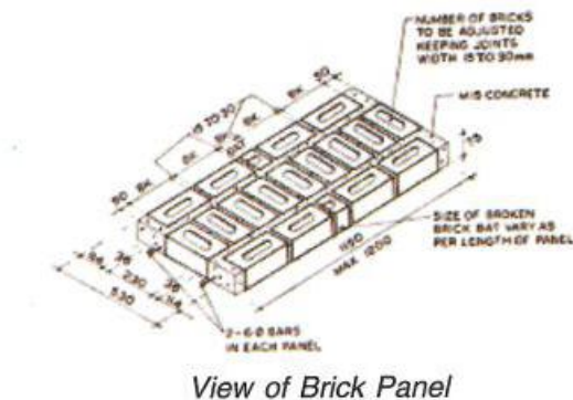
Fig. 4 Brick Panel
