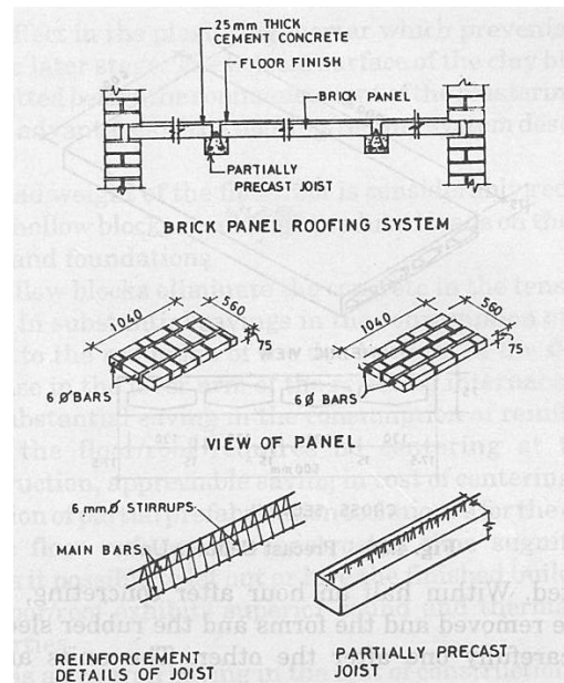
Fig. 5 Details of Precast Joist
