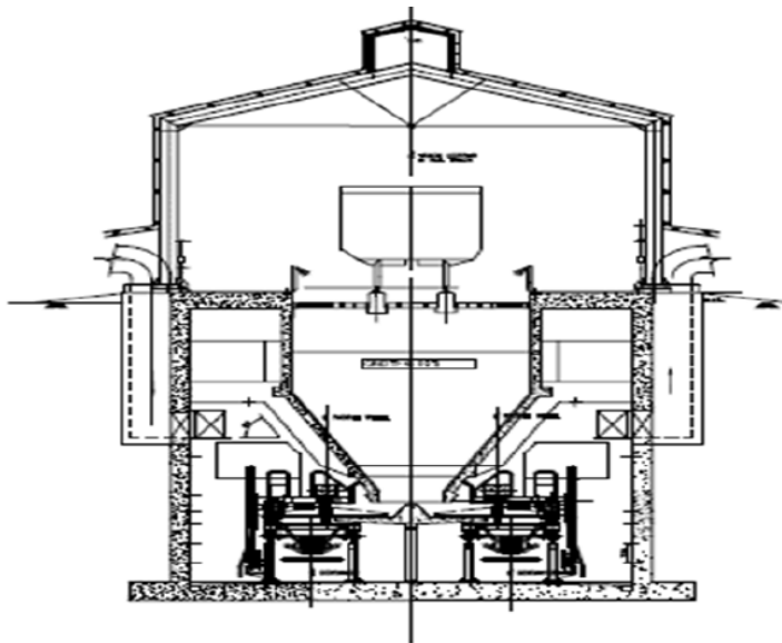
Typical Cross Section of Track Hopper
